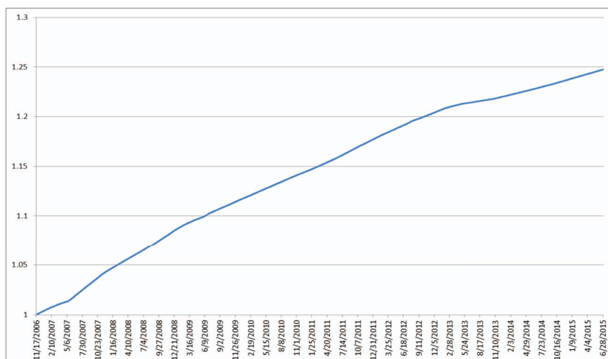
NAVPU Graph
